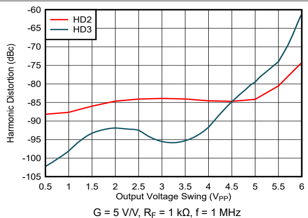
Figure 7-37. Harmonic Distortion vs Output Voltage Swing
