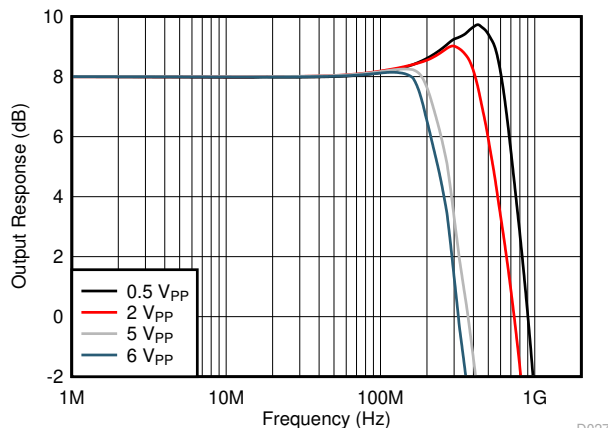
Figure 6-27. Noninverting Response vs Output Voltage
