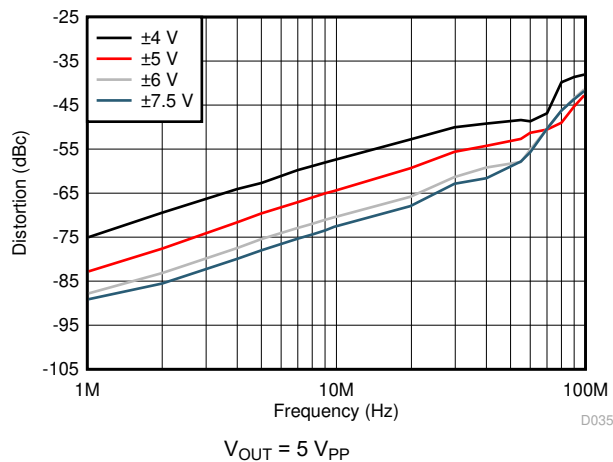
Figure 6-35. HD2 vs Supply Voltage
