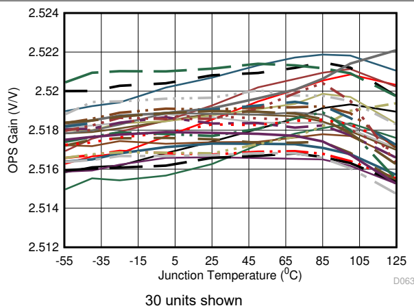
Figure 6-63. OPS Gain Over Temperature
