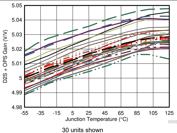
Figure 6-5. Gain vs Temperature
