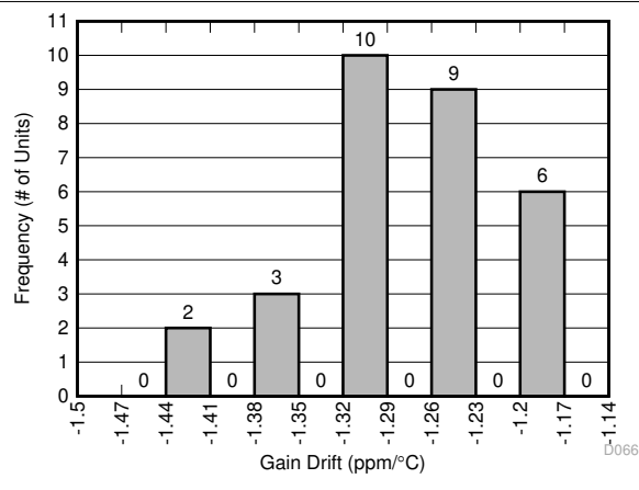
Figure 6-66. Midscale Buffer Gain Drift Histograms
