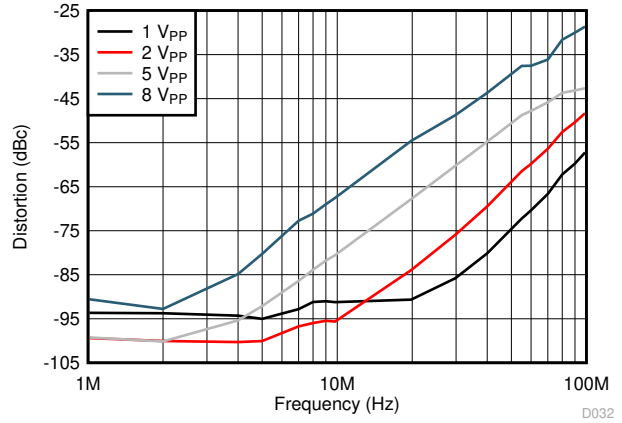
Figure 6-32. HD3 vs Output Voltage
