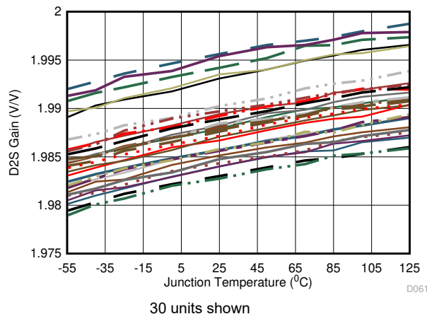
Figure 6-61. D2S Gain Over Temperature
