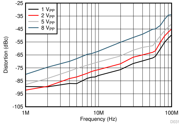
Figure 6-31. HD2 vs Output Voltage
