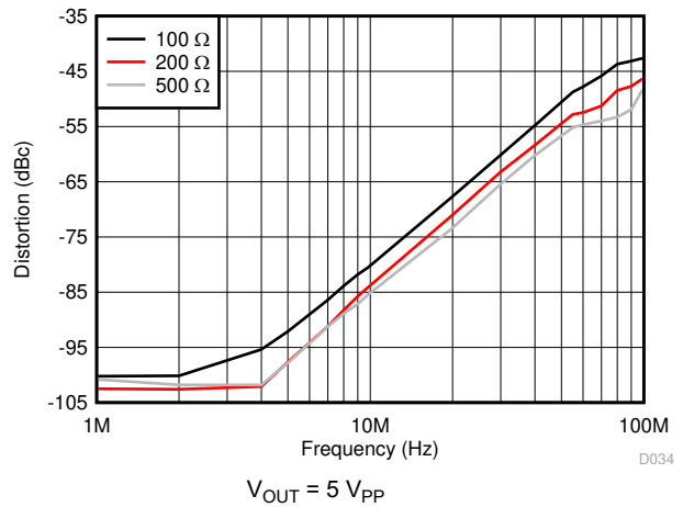
Figure 6-34. HD3 vs Load Resistance
