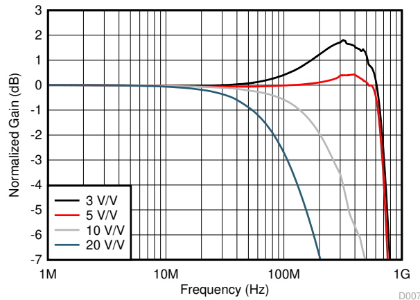
Figure 6-7. Small-Signal Frequency Response vs Gain
