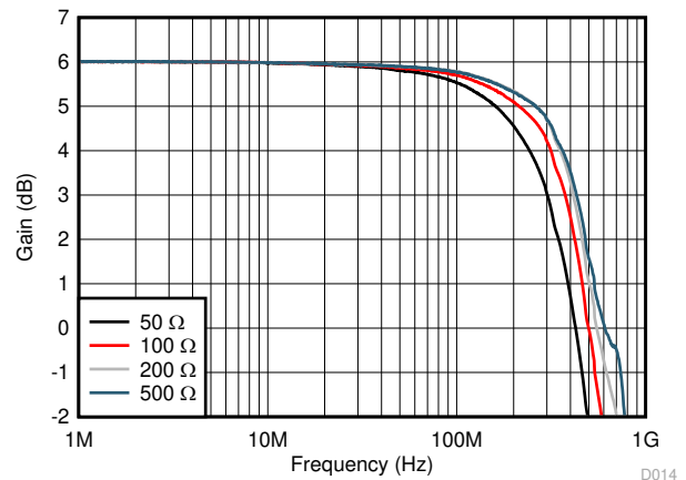
Figure 6-14. Frequency Response vs Load Resistance
