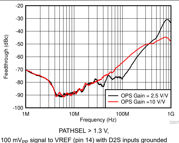
Figure 8-13. Forward Feedthrough With OPS Enabled, External Path Selected
