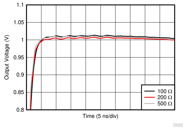
Figure 6-22. Large-Signal Pulse Settling Response vs Load Resistance
