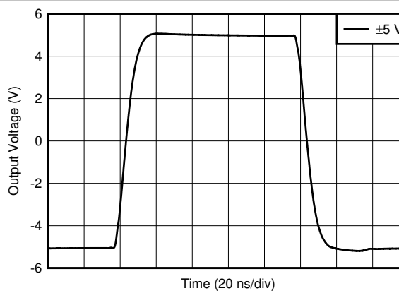
Figure 9-8. Pulse Response of the System With the Interstage Bessel Filter
