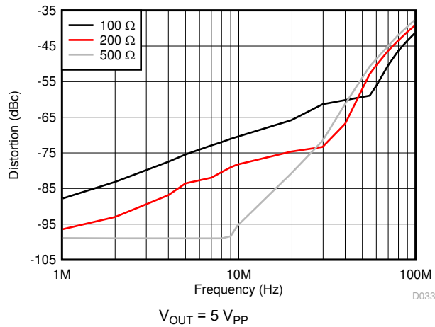
Figure 6-33. HD2 vs Load Resistance
