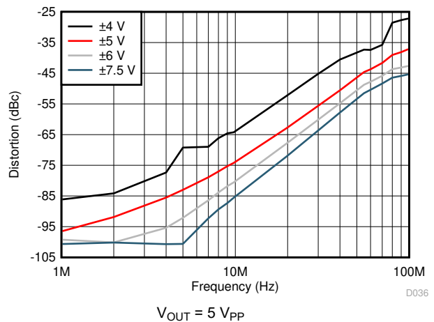
Figure 6-36. HD3 vs Supply Voltage
