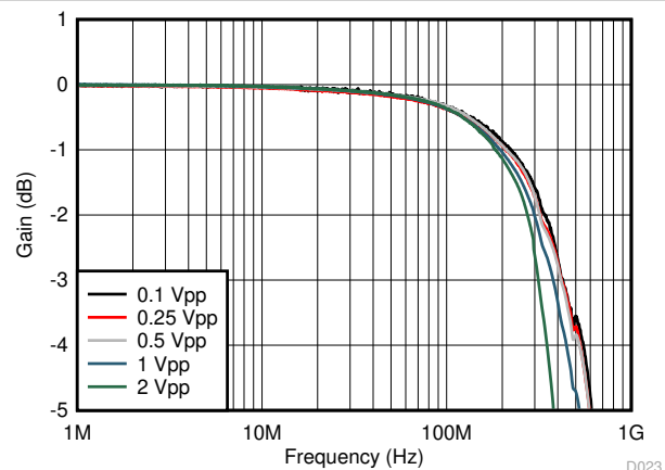
Figure 6-23. VREF Input Pin Frequency Response
