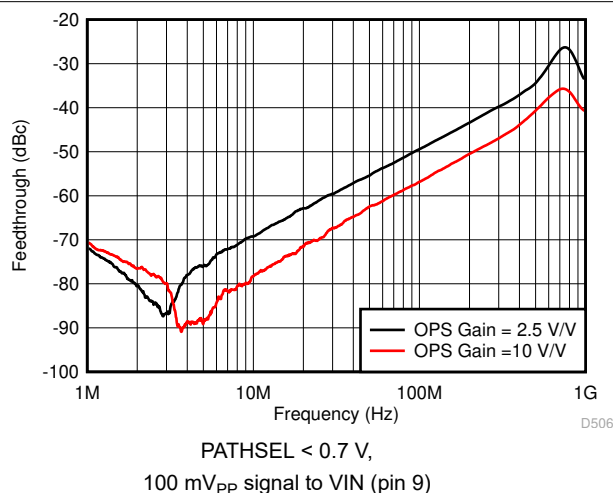
Figure 8-12. Forward Feedthrough With OPS Enabled, Internal Path Selected
