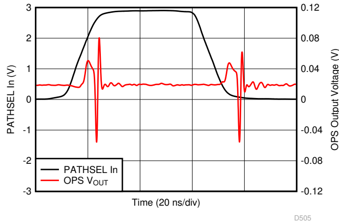
Figure 8-11. OPS Path-Select Switching Glitch
