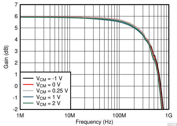
Figure 6-13. Frequency Response vs Input Common-Mode Voltage
