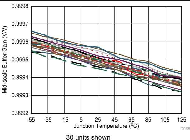
Figure 6-65. Midscale Buffer Gain Over Temperature
