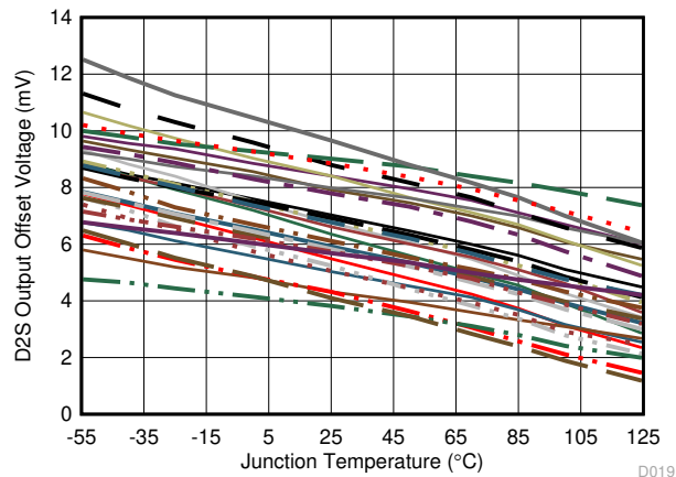
Figure 6-19. Output DC Offset Voltage vs Die Temperature
