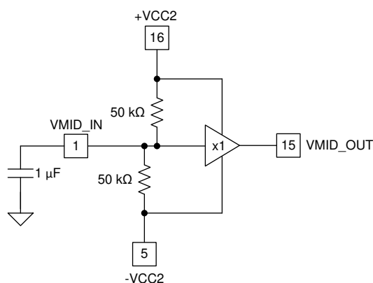
Figure 8-5. Midscale Buffer Noise Model
