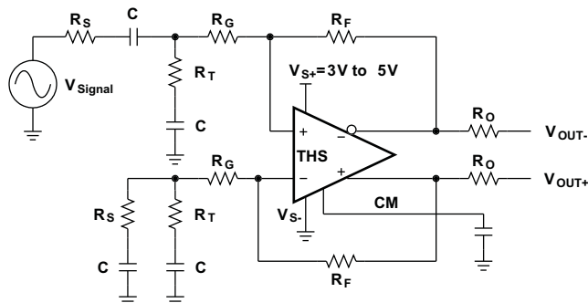
Figure 65. THS4513 AC Coupled Single-Supply
