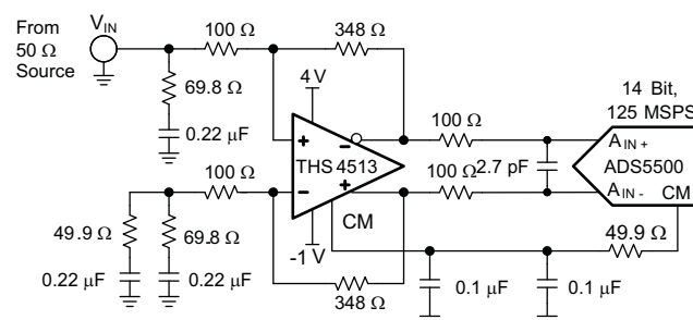
Figure 66. THS4513 + ADS5500 Circuit
