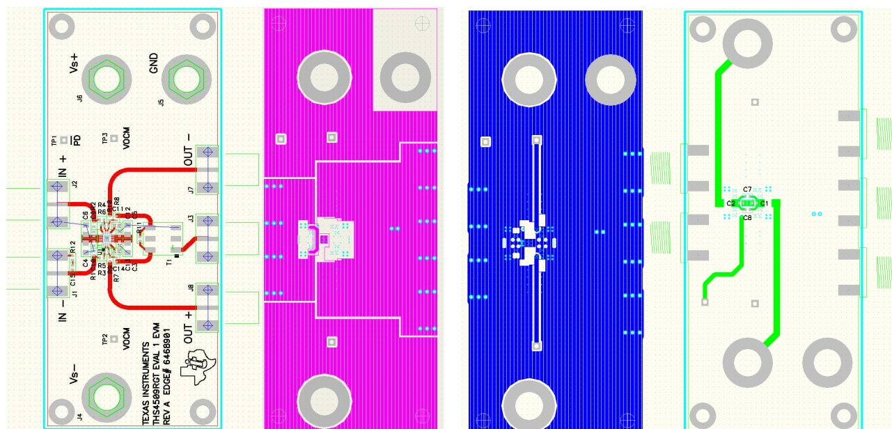
Figure 70. THS4513 EVAL1 EVM Layer 1 Through 4
