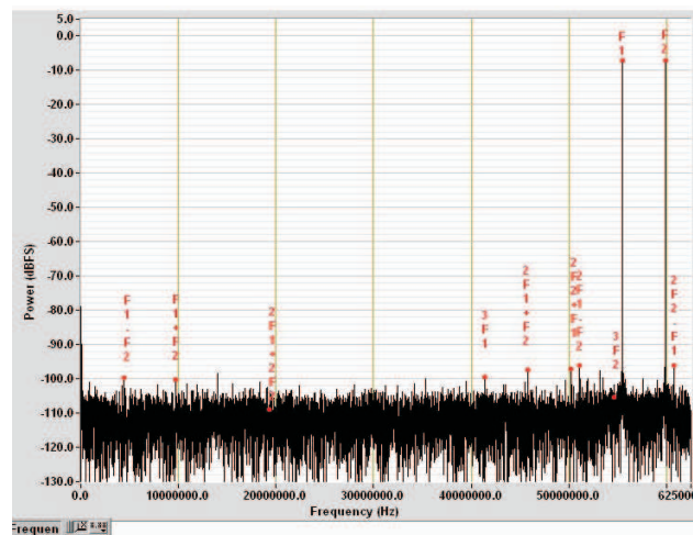
Figure 67. THS4513 + ADS5500 2-Tone FFT With 65 MHz and 70 MHz Input
