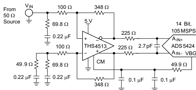
Figure 68. THS4513 + ADS5424 Circuit
