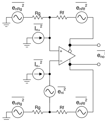
Figure 7-10. FDA Noise-Analysis Circuit
