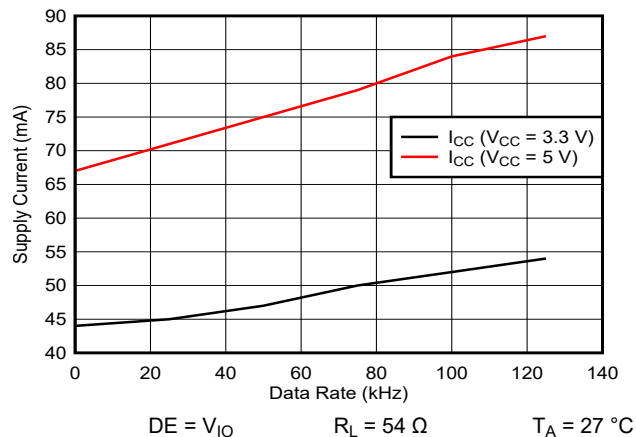
Figure 5-14. THVD2410V Supply Current vs Signal Rate
