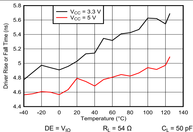
Figure 5-11. THVD2450V 50Mbps Driver rise or fall time vs Temperature
