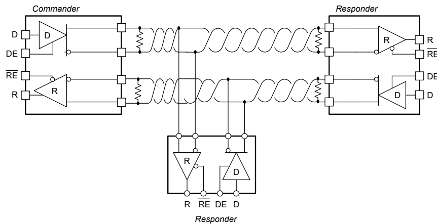
Figure 8-2. Typical RS-485 Network with Full-Duplex transceivers
