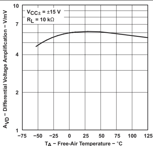
Figure 6-5. Differential Voltage Amplification vs Free-Air Temperature
