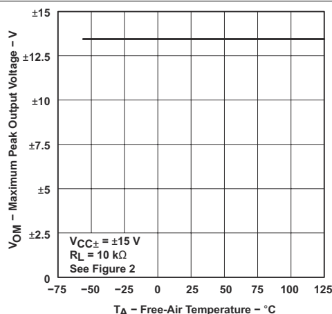
Figure 6-2. Maximum Peak Output Voltage vs Free-Air Temperature
