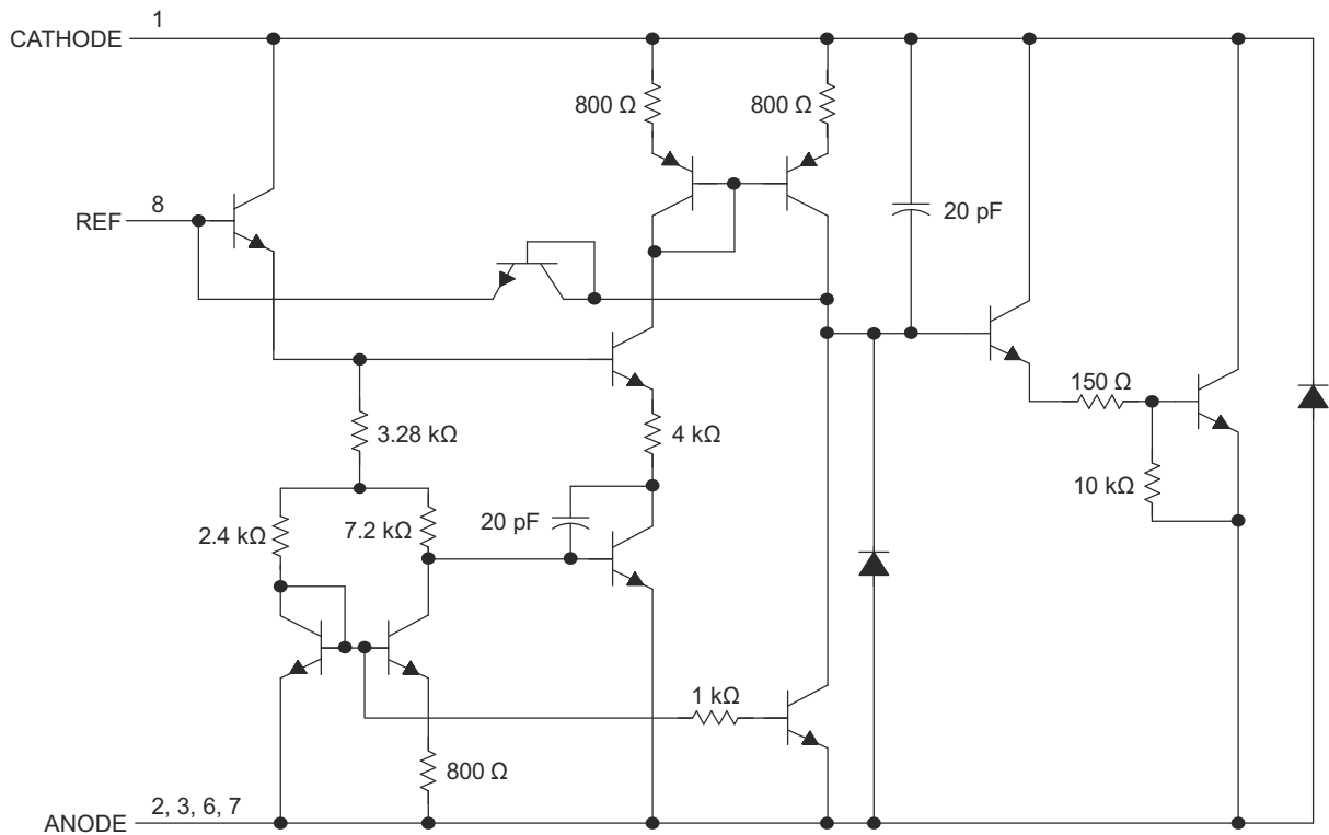
Figure 8-2. Equivalent Schematic
