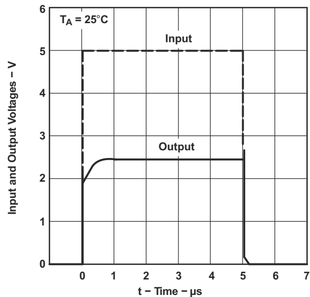
Figure 6-14. Pulse Response
