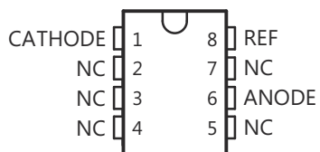
Figure 5-1. JG Package 8-Pin CDIP Top View
