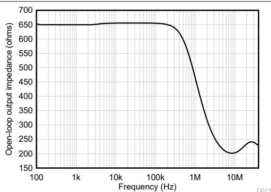
Figure 5-13. Open-Loop Output Impedance vs Frequency, New Die
