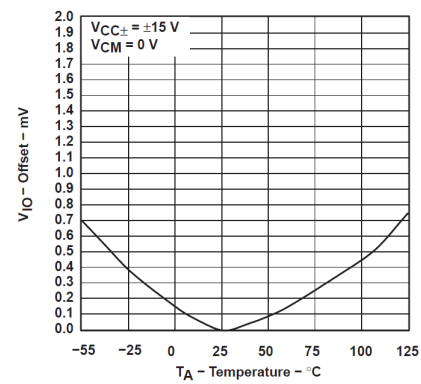
Figure 5-6. Offset Voltage Drift vs Temperature, Old Die
