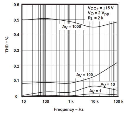
Figure 5-2. Total Harmonic Distortion vs Frequency, Old Die
