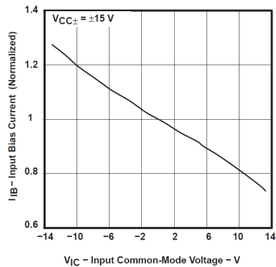
Figure 5-7. Normalized Input Bias Current vs Input Common-Mode Voltage, Old Die
