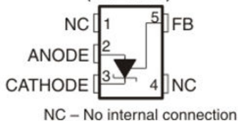
Adjustable...DCK (SC-70) PACKAGE (TOP VIEW)
