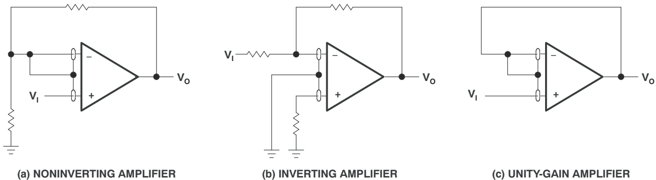
Figure 7-5. Guard-Ring Schemes
