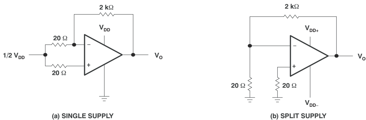
Figure 6-2. Noise-Test Circuit
