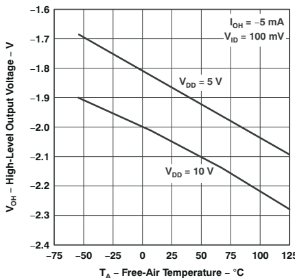
Figure 5-8. High-Level Output Voltage vs Free-Air Temperature
