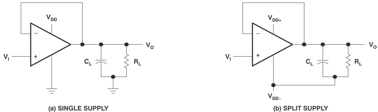
Figure 6-1. Unity-Gain Amplifier
