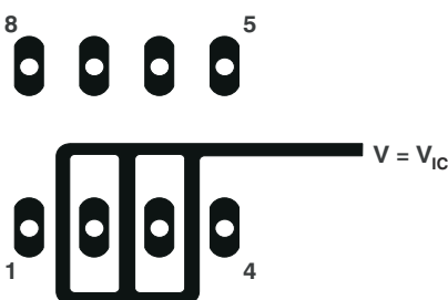
Figure 6-4. Isolation Metal Around Device Inputs (P package)
