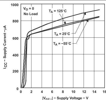
Figure 5-36. TLE2024xM Supply Current vs Supply Voltage
