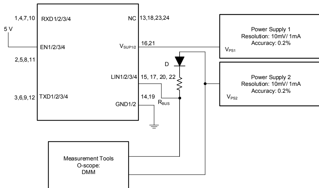
Figure 8-5. V<sub>SUP</sub>_NON_OP
