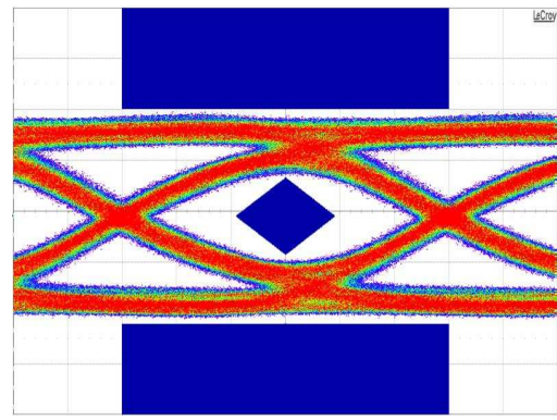
Figure 7. Transmitter Output (8-Inch FR-4 Trace)
