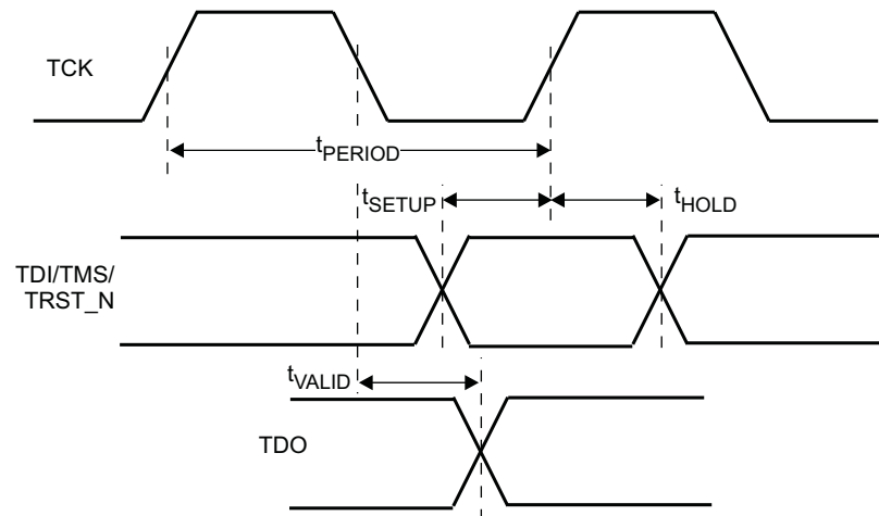
Figure 5. JTAG Timing
