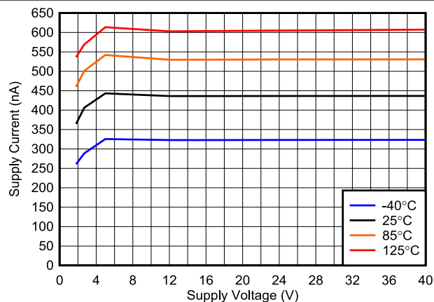
Figure 6-22. Supply Current vs. Supply Voltage (Output High), Open Drain
