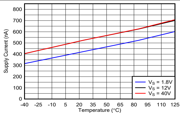
Figure 6-24. Supply Current vs. Temperature (Output High), Push-Pull
