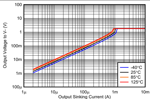
Figure 6-14. Output Voltage vs. Output Sinking Current, 1.8 V
