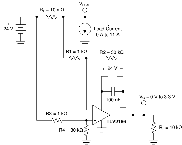
Figure 46. TLV2186 High-Side Current-Monitor Simulation Schematic
