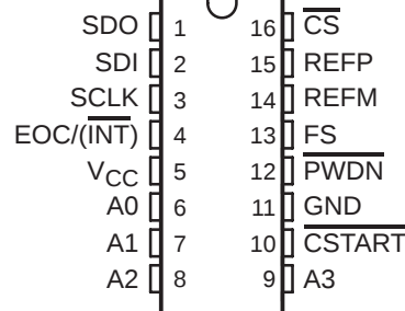
TLV2544Q . . . D PACKAGE (TOP VIEW)
