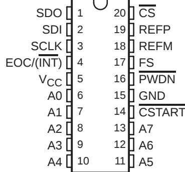
TLV2548Q . . . DW PACKAGE (TOP VIEW)
