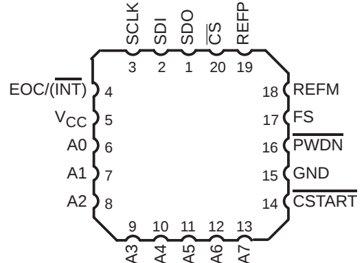
TLV2548M . . . FK PACKAGE (TOP VIEW)
