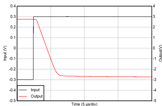
Figure 5-39. Positive Overload Recovery
