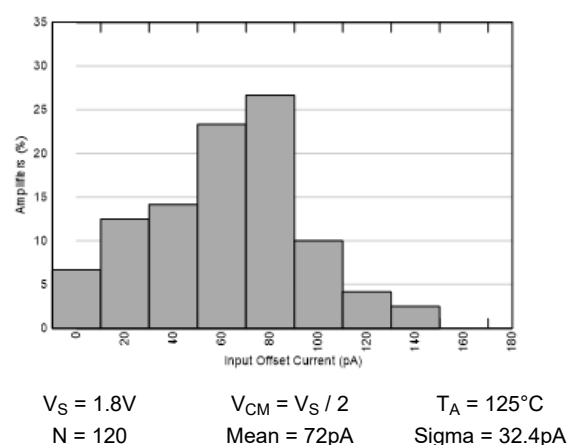
Figure 5-12. Input Offset Current Distribution
