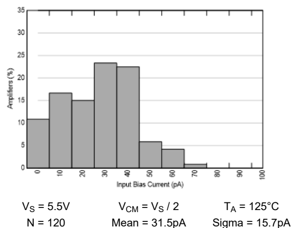
Figure 5-8. Input Offset Current Distribution
