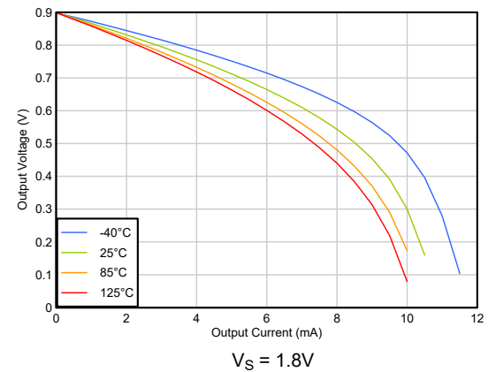
Figure 5-22. Output Voltage Swing vs Output Current (Sourcing)
