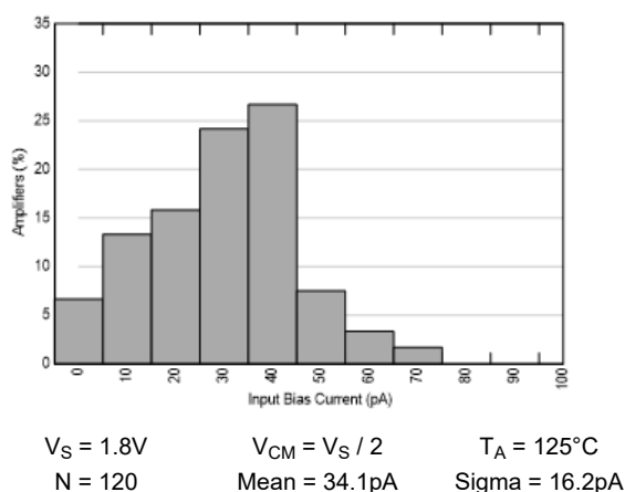
Figure 5-11. Input Bias Current Distribution
