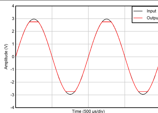
Figure 5-38. No Phase Reversal
