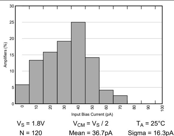
Figure 5-9. Input Bias Current Distribution
