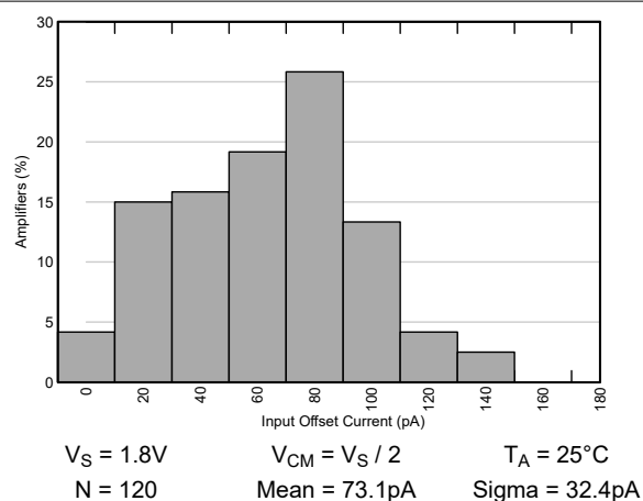
Figure 5-10. Input Offset Current Distribution
