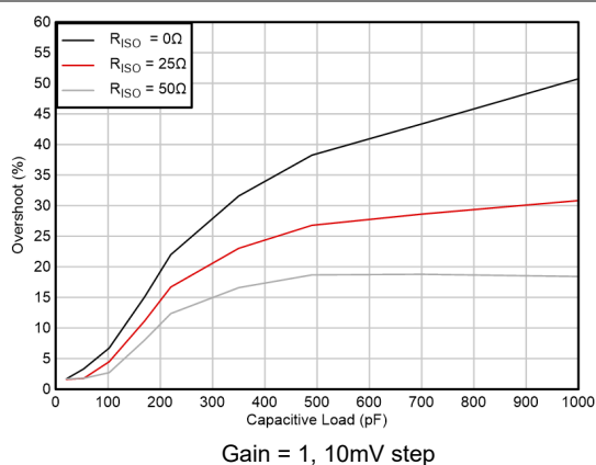
Figure 5-37. Small-Signal Overshoot vs Capacitive Load
