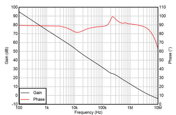
Figure 5-18. Open-Loop Gain and Phase vs Frequency
