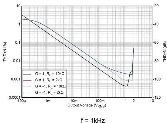
Figure 5-31. THD+N vs Output Amplitude
