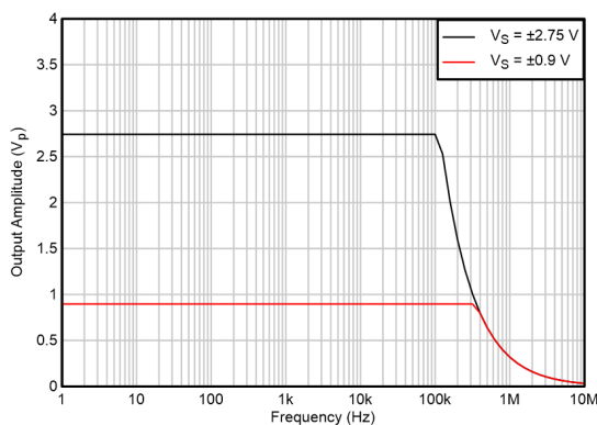
Figure 5-47. Maximum Output Voltage vs Frequency
