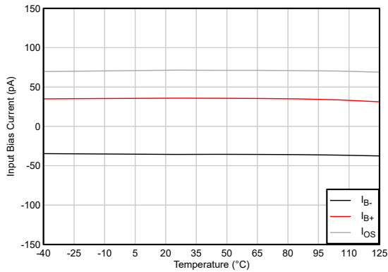
Figure 5-17. Input Bias Current and Offset Current vs Temperature
