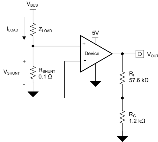
Figure 7-3. TLVx825 in a Low-Side, Current-Sensing Application
