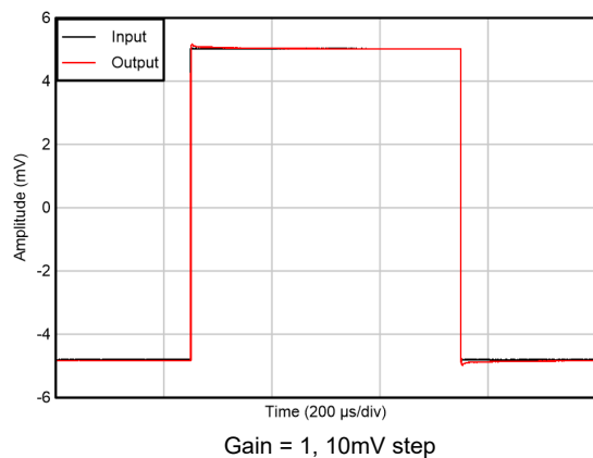
Figure 5-41. Small-Signal Step Response
