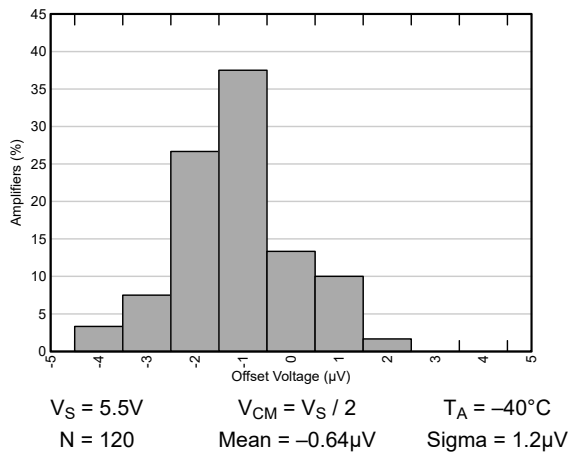
Figure 5-3. Offset Voltage Distribution
