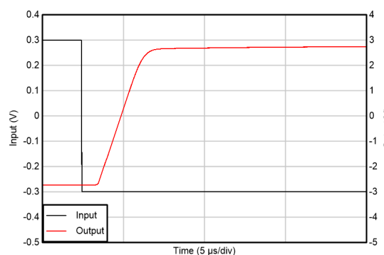
Figure 5-40. Negative Overload Recovery
