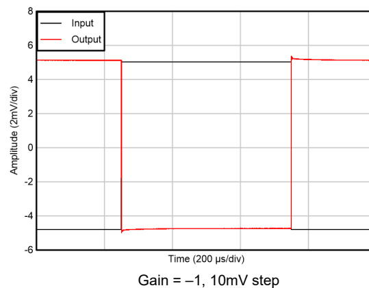
Figure 5-42. Small-Signal Step Response
