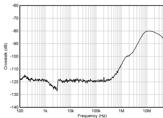
Figure 5-49. Channel Separation
