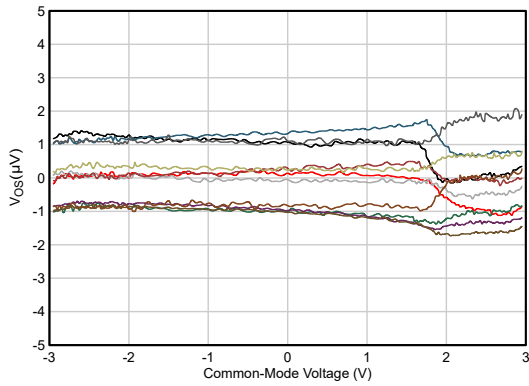
Figure 5-13. Offset Voltage vs Common-Mode Voltage
