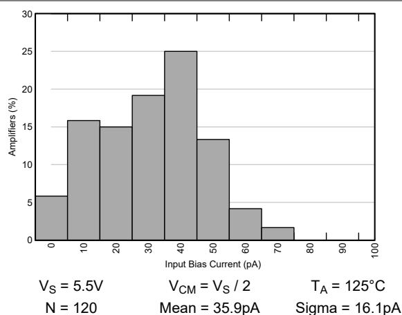
Figure 5-7. Input Bias Current Distribution
