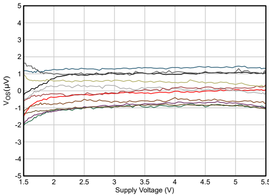
Figure 5-15. Offset Voltage vs Supply Voltage
