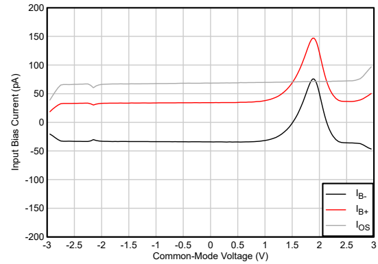
Figure 5-16. Input Bias Current vs Common-Mode Voltage
