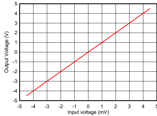
Figure 7-5. High Gain Amplifier Results
