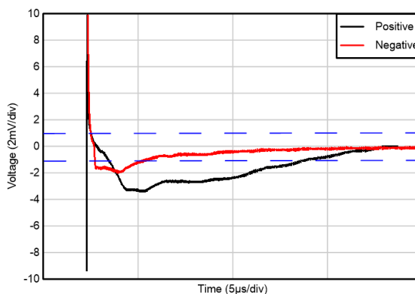
Figure 5-38. Settling Time
