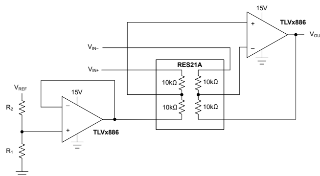
Difference Amplifier
