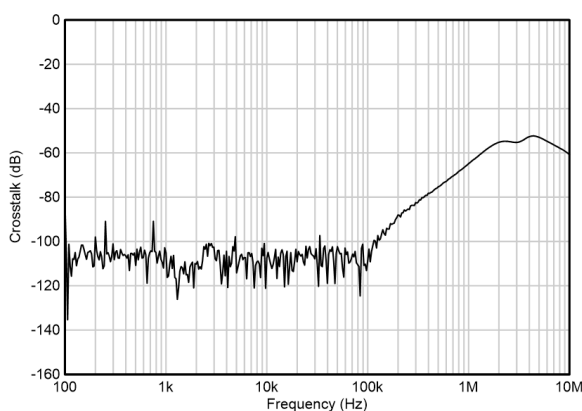
Figure 5-42. Channel Separation
