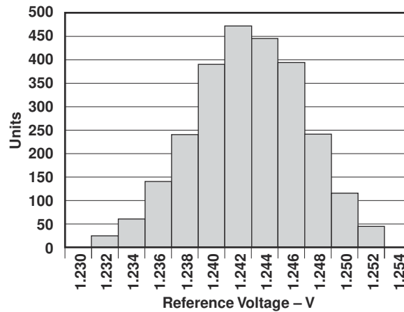
Figure 6-17. REFERENCE VOLTAGE DISTRIBUTION
