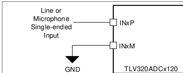
Figure 8-14. Single-Ended, DC-Coupled Input Connection
