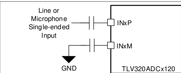
Figure 8-15. Single-Ended, AC-Coupled Input Connection
