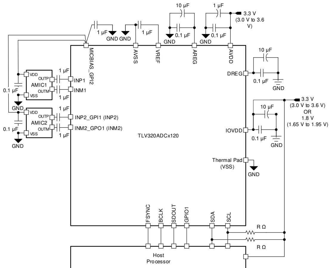
Figure 9-1. Two-Channel Analog Microphone Recording Diagram
