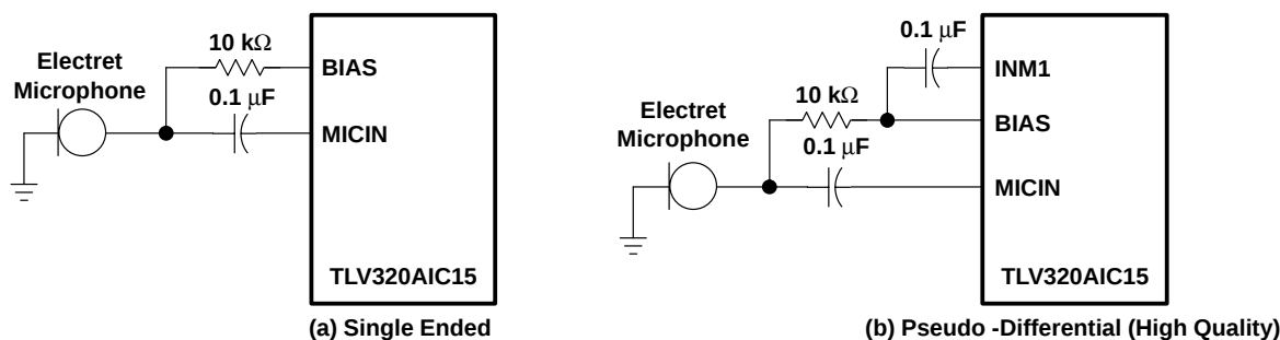
Figure 3–1. Microphone Interface
