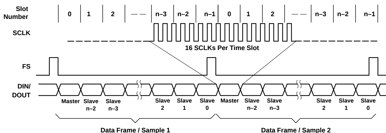
Figure 3-15. Standard Operation/Continuous Data Transfer Mode: Stand-Alone Timing
