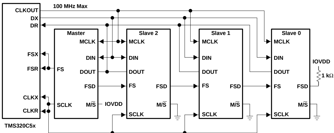
Figure 3–7. Cascade Connection (To DSP Interface)
