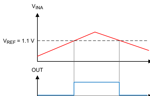
Figure 7-8. Overcurrent Results
