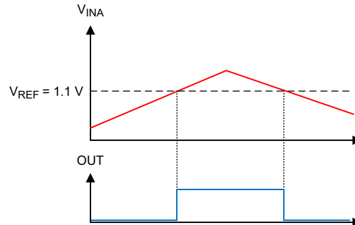
Figure 7-8. overcurrent Results
