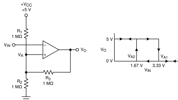
Figure 7-3. TLV321x in an Inverting Configuration With Hysteresis
