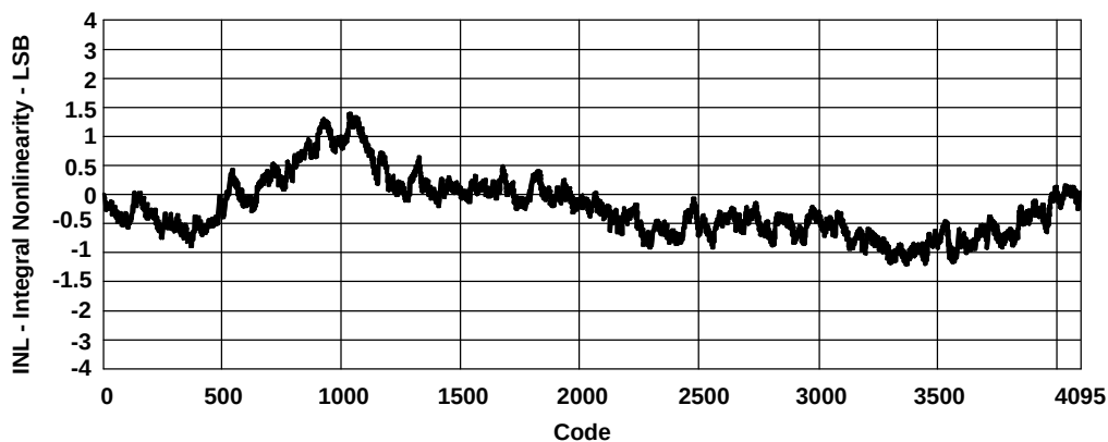
Figure 8. Integral Nonlinearity
