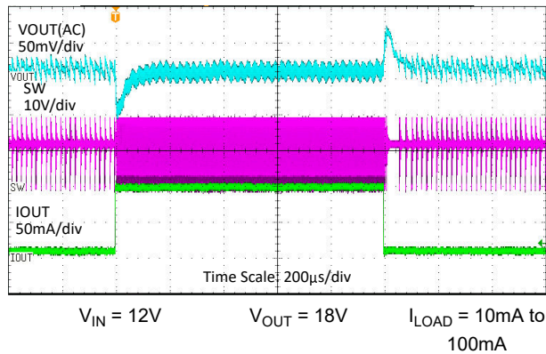
Figure 7-12. Load Transient
