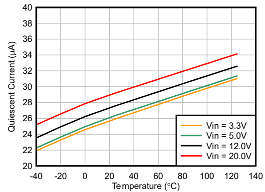
Figure 5-4. Quiescent Current vs Temperature
