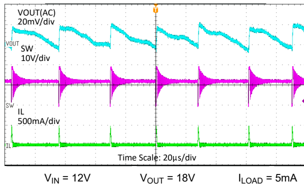
Figure 7-10. Switching Waveforms in Steady State
