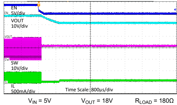
Figure 7-9. Shutdown by EN waveforms
