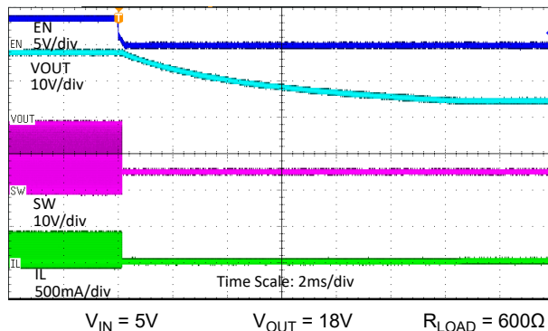
Figure 7-3. Shutdown by EN waveforms
