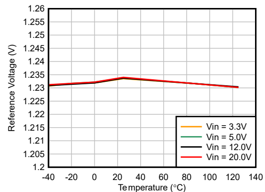
Figure 5-6. Reference Voltage vs Temperature
