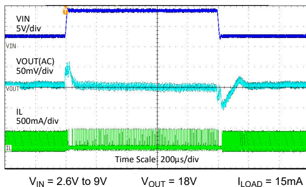
Figure 7-7. Line Transient
