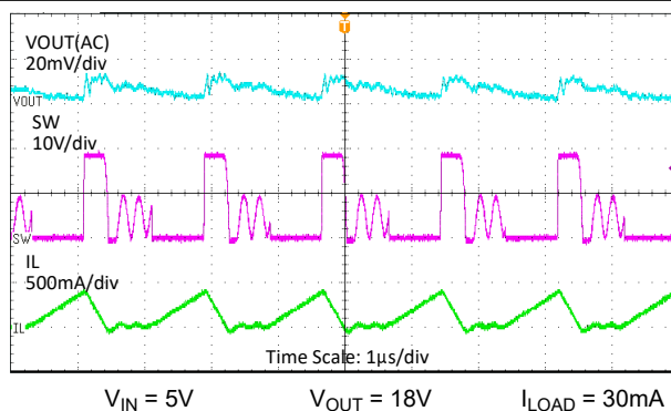
Figure 7-5. Switching Waveforms in Steady State
