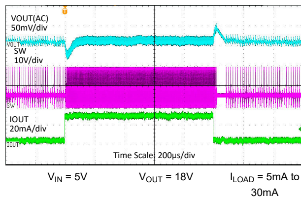
Figure 7-6. Load Transient
