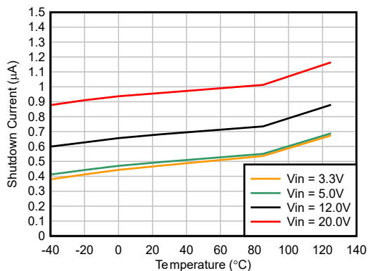
Figure 5-5. Shutdown Current vs Temperature
