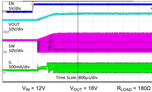
Figure 7-8. Start-up by EN waveforms
