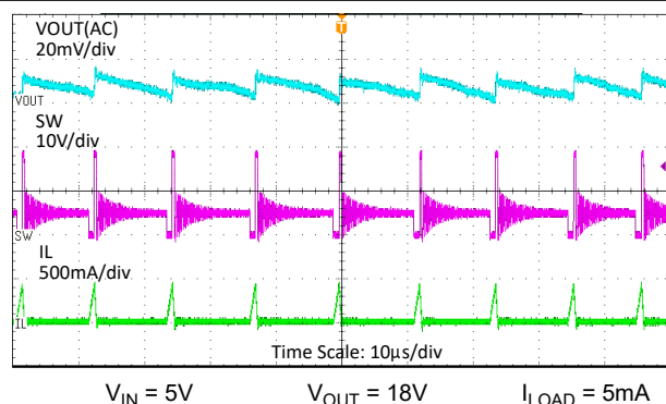
Figure 7-4. Switching Waveforms in Steady State
