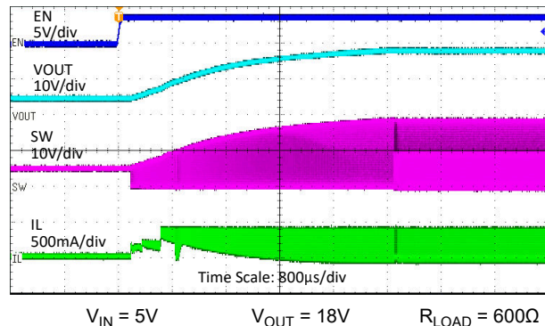
Figure 7-2. Start-up by EN Waveforms
