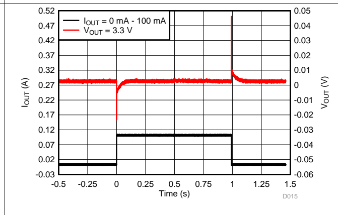
Figure 16. Load Transient
