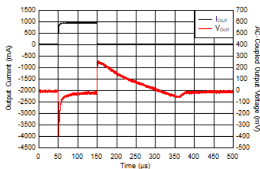
Figure 7-4. I_{OUT} Transient From 1 mA to 1 A
