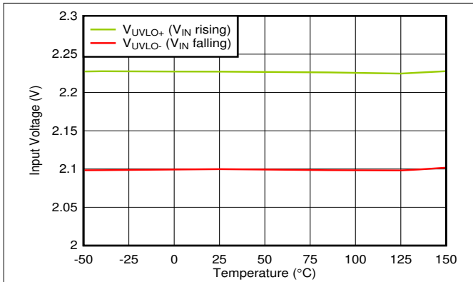
Figure 7-25. UVLO Thresholds vs Temperature
