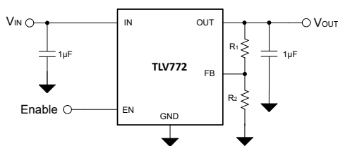
Typical Application Circuit
