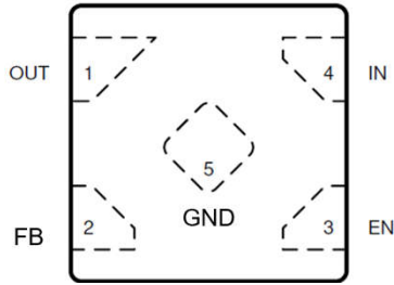
Figure 4-1. DQN Package, 1mm × 1mm, 5-Pin X2SON (Top View)
