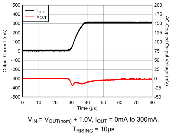
Figure 5-11. Load Transient
