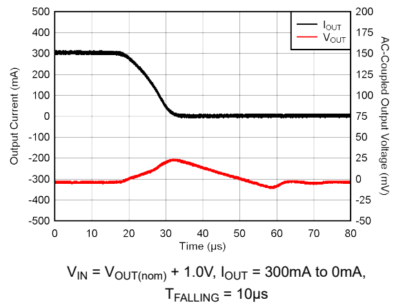
Figure 5-12. Load Transient
