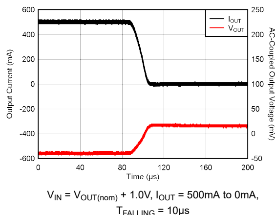
Figure 5-13. Load Transient
