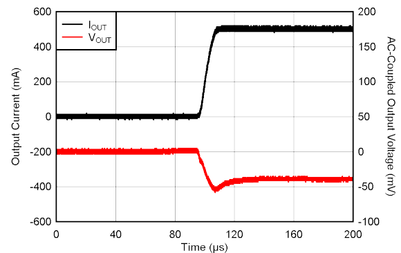
Figure 5-10. Current Limit
