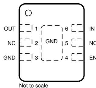
Figure 4-2. DRV Package, 6-Pin WSON (Top View)
