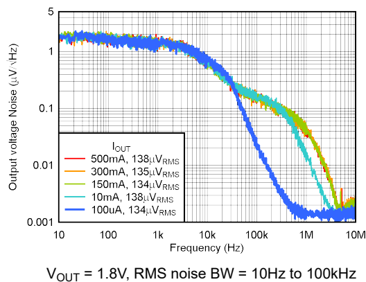
Figure 5-17. Noise
