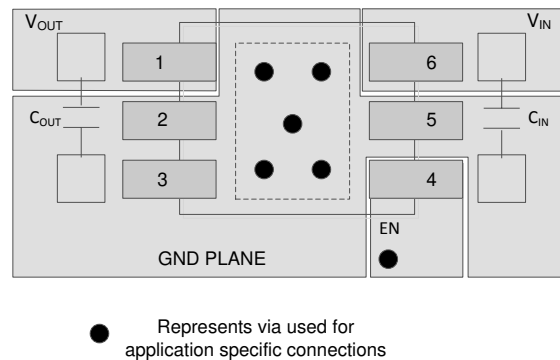
Figure 7-5. DRV Package (WSON) Typical Layout
