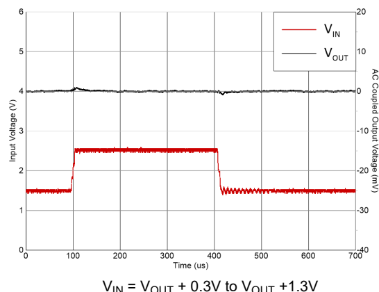
Figure 5-14. Line Transient
