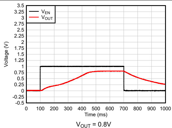
Figure 5-14. Start-Up
