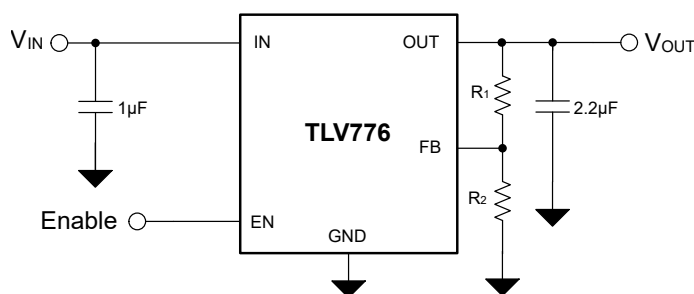
Figure 7-1. TLV776 Typical Application
