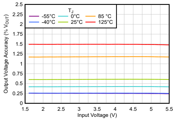
Figure 5-1. Output Voltage Accuracy vs V_{IN}
