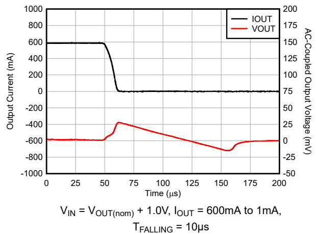
Figure 5-10. Load Transient
