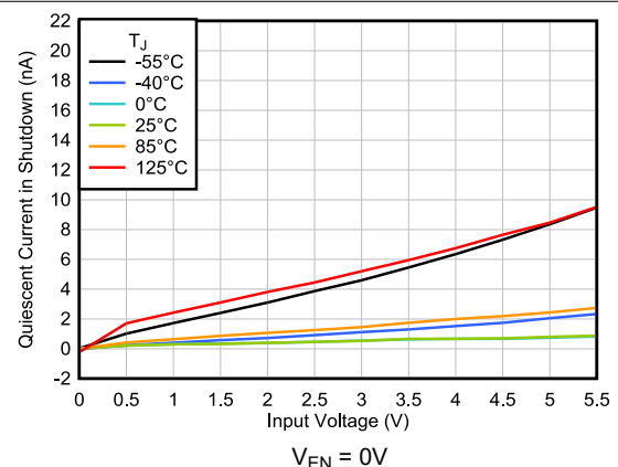
Figure 5-6. Shutdown Current vs V_{IN}
