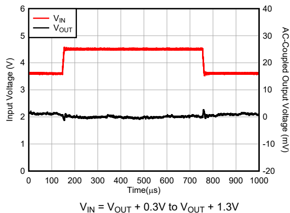
Figure 5-11. Line Transient
