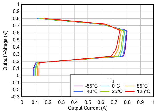
Figure 5-7. Current Limit
