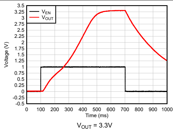
Figure 5-13. Start-Up
