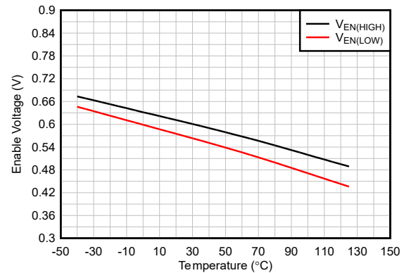
Figure 5-8. Enable Logic Threshold vs Temperature
