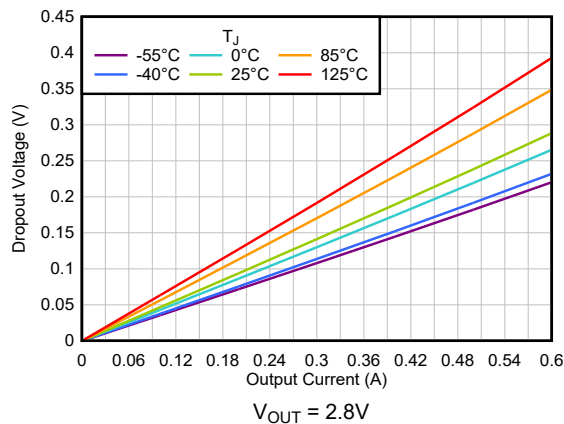
Figure 5-3. Dropout Voltage vs I_{OUT}
