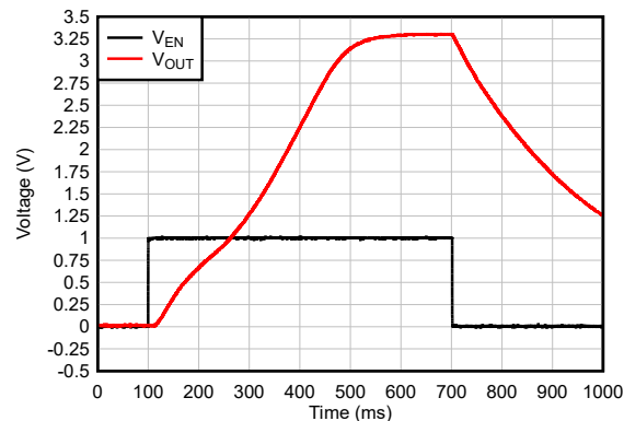
Figure 7-2. Start-Up
