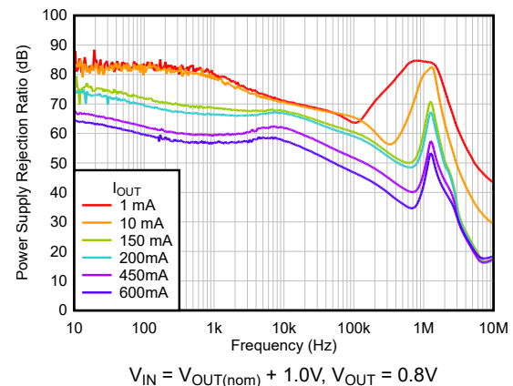
Figure 5-12. PSRR vs Frequency
