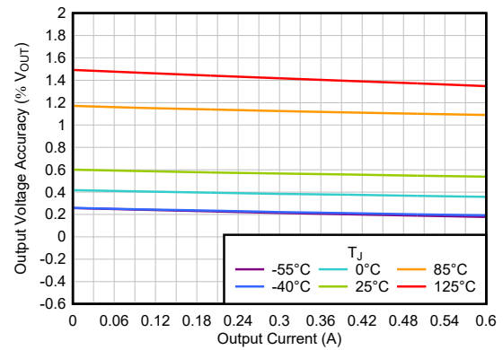
Figure 5-2. Output Voltage Accuracy vs I_{OUT}
