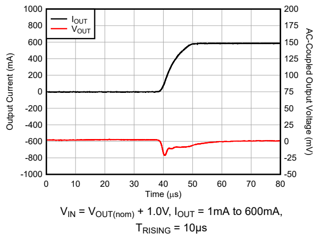
Figure 5-9. Load Transient
