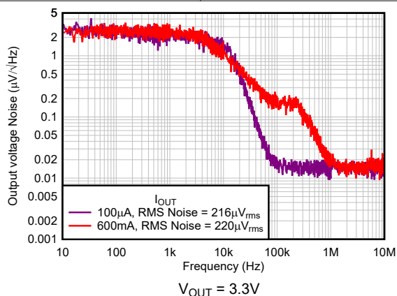
Figure 5-15. Noise
