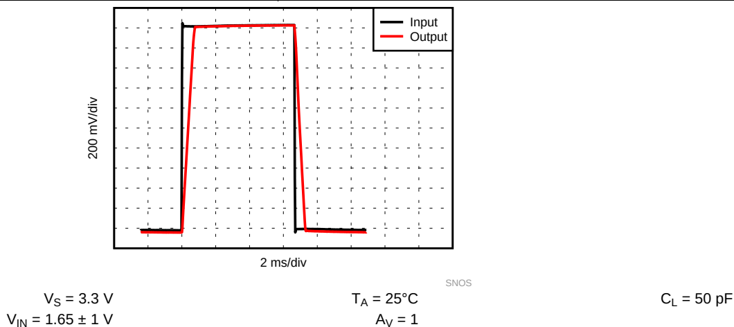
Figure 29. Large Signal Pulse Response, 3.3 V
