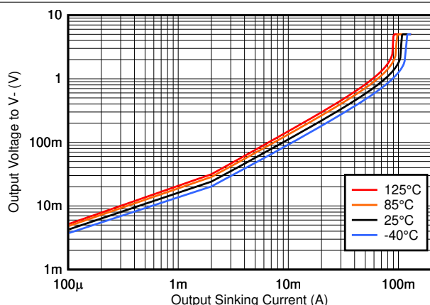
Figure 5-11. Output Sinking Current vs. Output Voltage, 5V
