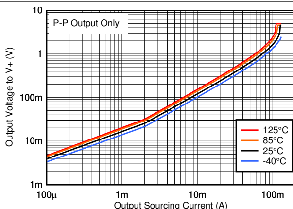
Figure 5-12. Output Sourcing Current vs. Output Voltage, 5V
