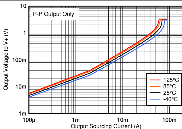
Figure 5-10. Output Sourcing Current vs. Output Voltage, 3.3V
