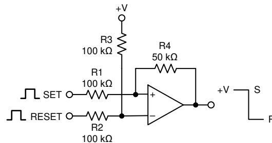
Figure 7-16. Bi-Stable Multivibrator
