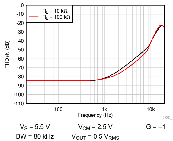
Figure 6-24. THD + N vs Frequency
