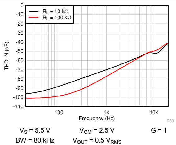
Figure 6-23. THD + N vs Frequency
