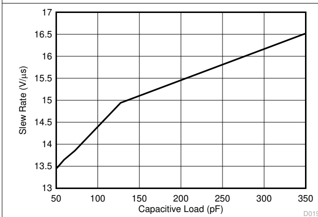
Figure 6-21. Slew Rate vs Capacitive Load
