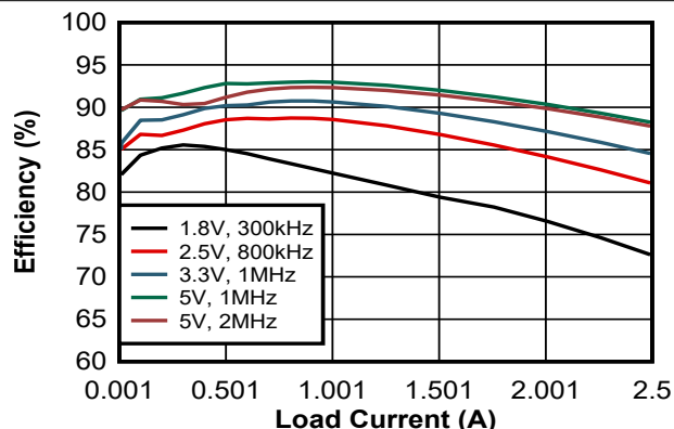
Figure 8-4. 12VIN Efficiency (Linear)
