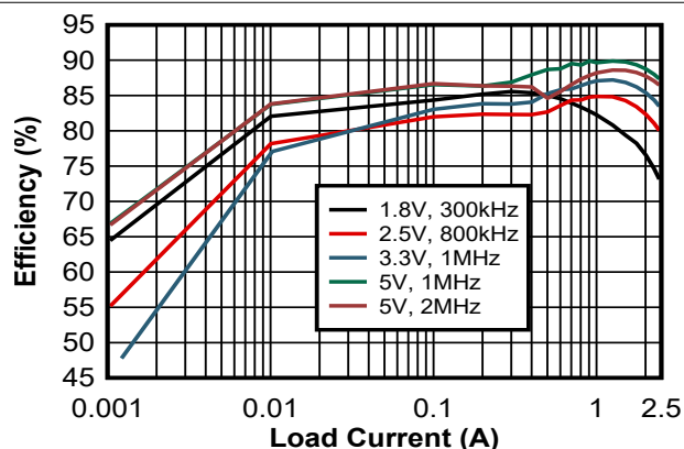
Figure 8-6. 24VIN Efficiency (Log)
