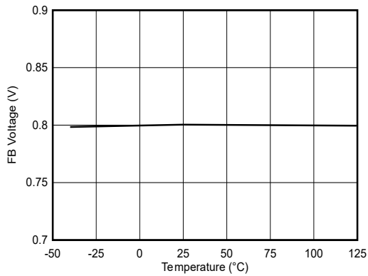
Figure 5-1. Feedback Voltage
