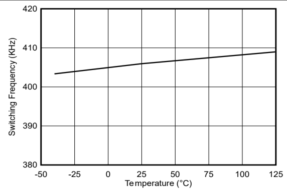
Figure 5-6. f_{SW} 400kHz
