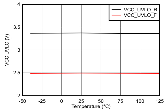
Figure 5-4. VCC UVLO
