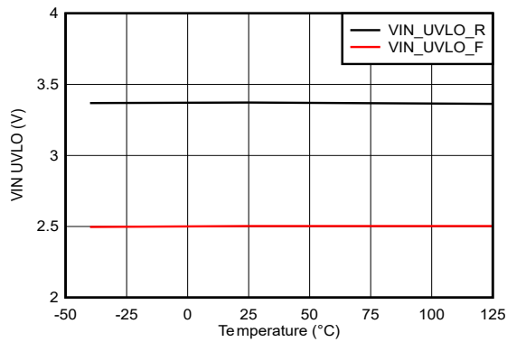
Figure 5-3. Enable UVLO
