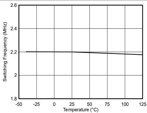
Figure 5-5. f_{SW} 2.2MHz
