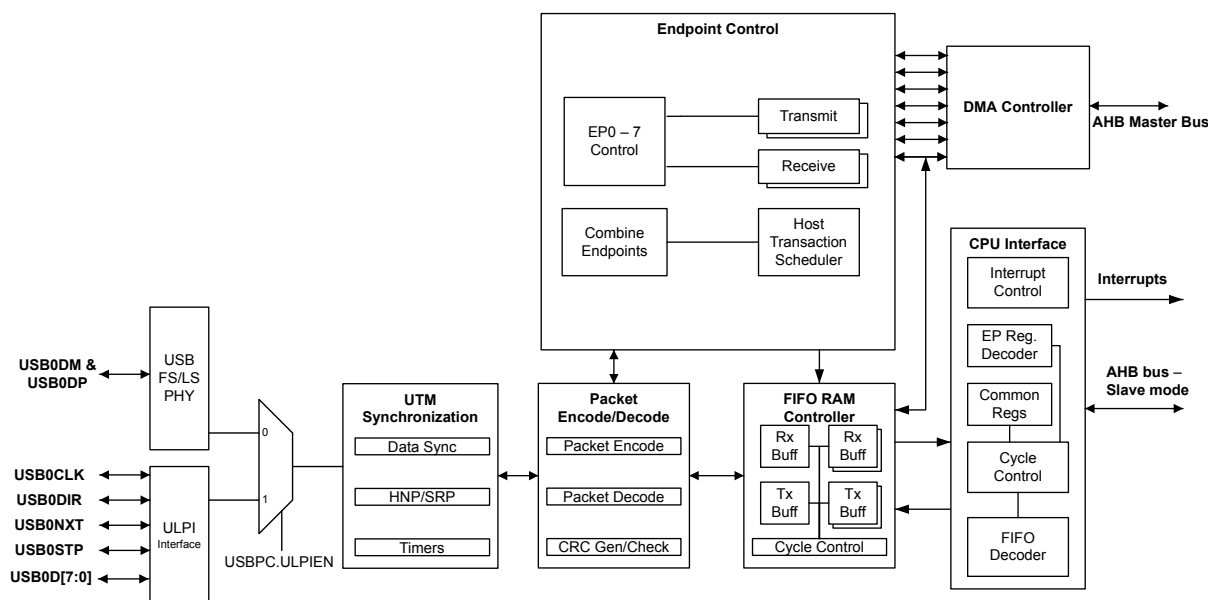
Figure 23-1. USB Module Block Diagram
