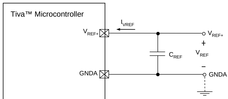
Figure 29-28. ADC External Reference Filtering
