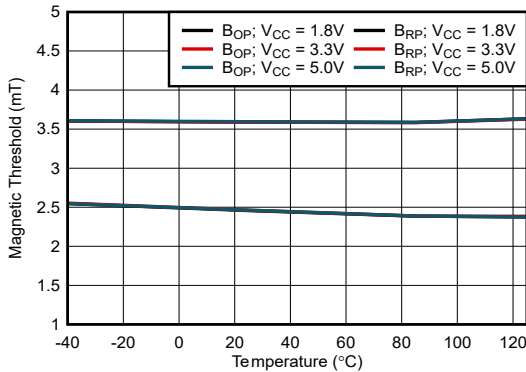
Figure 6-3. 3.5mT B_{OP} : Thresholds vs Temperature
