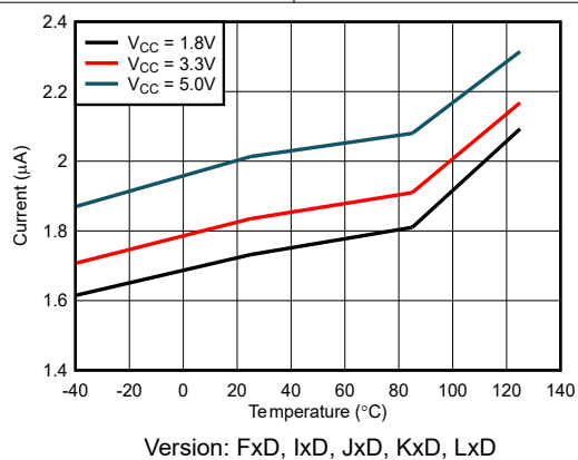
Figure 6-9. 20Hz I CCAVG vs Temperature
