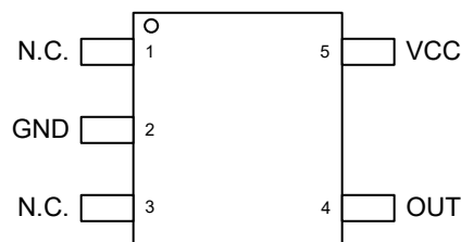
Figure 5-3. DBV Package 5-Pin Top View
