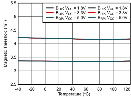
Figure 6-4. 4.1mT B_{OP} : Thresholds vs Temperature
