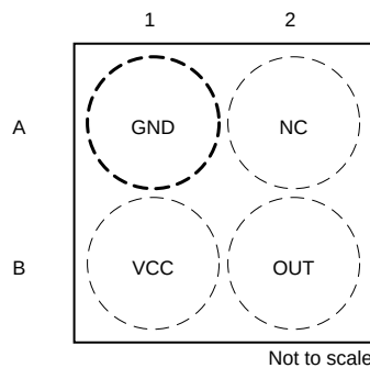
Figure 5-1. YBK and YBH Package 4-Pin DSBGA (Omnipolar) Top View
