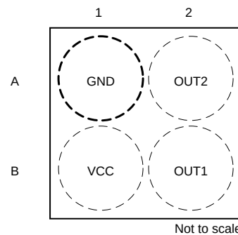
Figure 5-2. YBK and YBH Package 4-Pin DSBGA (Dual-Unipolar) Top View
