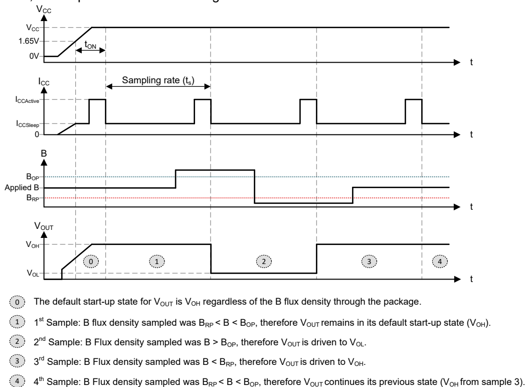
Figure 7-7. Timing and Output Diagram
