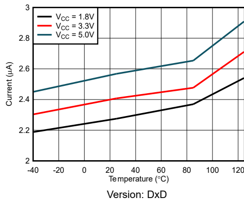
Figure 6-8. 20Hz I CCAVG vs Temperature
