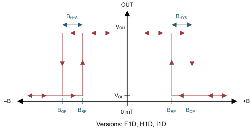
Figure 7-5. Omnipolar Active Low Functionality
