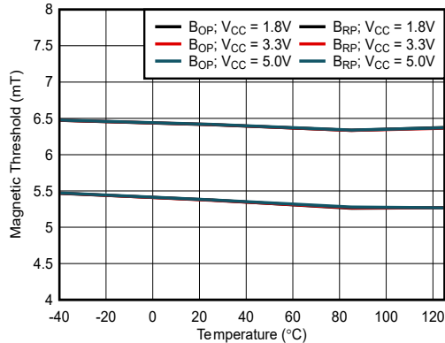
Figure 6-5. 6.3mT B_{OP} : Thresholds vs Temperature
