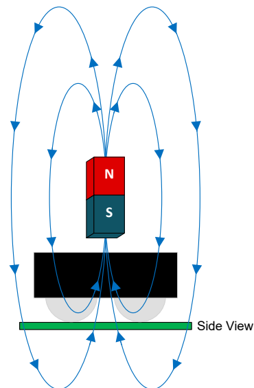
Figure 7-4. Positive Magnetic Flux Density: Magnet In-Line
