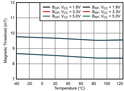
Figure 6-6. 9.5mT B_{OP} : Thresholds vs Temperature
