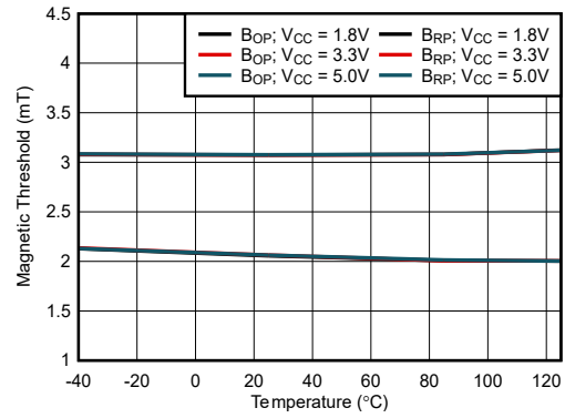
Figure 6-2. 3mT B_{OP} , 2.1mT B_{RP} : Thresholds vs Temperature
