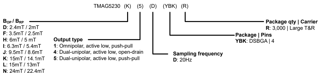
Figure 9-1. Device Nomenclature
