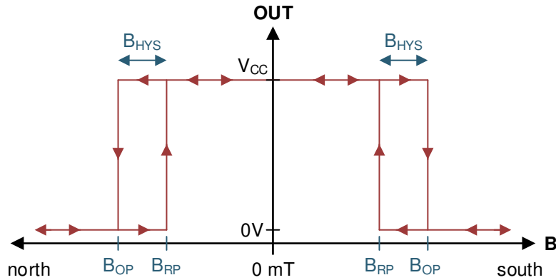
Figure 8-3. Omnipolar Functionality
