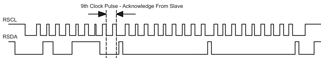
Figure 35. Bus-R Waveform
