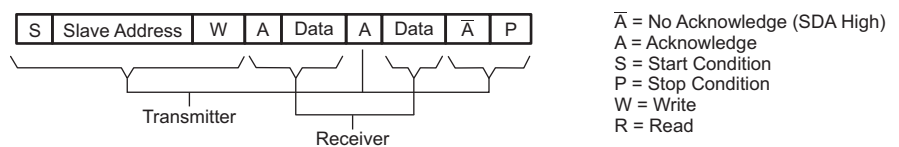
Figure 44. I²C Read Cycle
