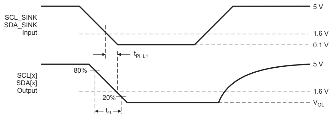
Figure 11. Source-Side Output AC Measurements
