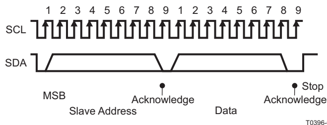
Figure 41. I²C Address, Data Cycle(s), and Stop
