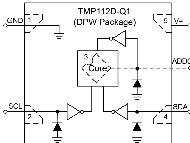
Figure 7-3. Equivalent Internal ESD Circuitry (X2SON Package)
