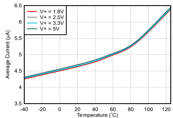
Figure 6-12. Average Quiescent Current vs Temperature
