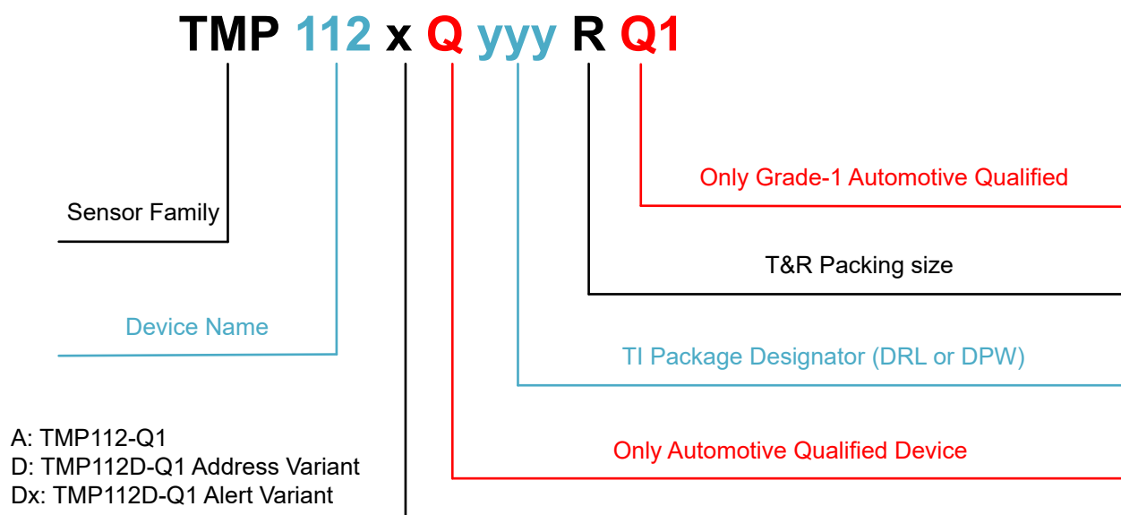
Figure 4-1. TMP112-Q1 and TMP112D-Q1 Device Nomenclature
