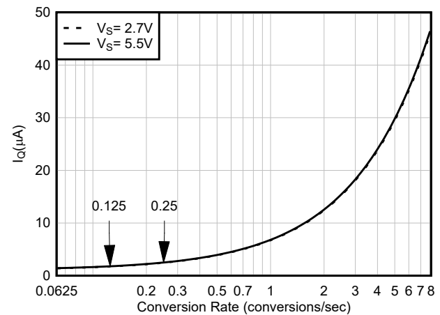
Figure 6-17. Quiescent Current vs Conversion Rate (New Chip)
