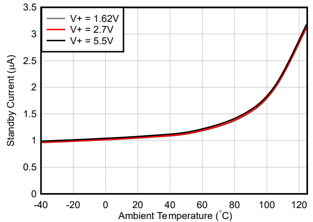
Figure 6-32. Standby Current vs Temperature
