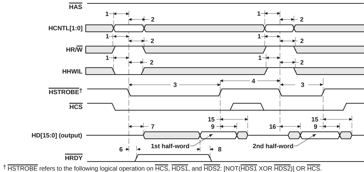
Figure 7-32. HPI16 Read Timing ( \overline{HAS} Not Used, Tied High)
