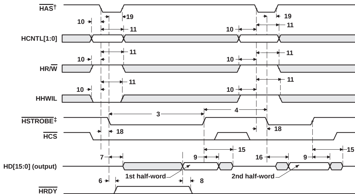
Figure 7-33. HPI16 Read Timing ( \overline{HAS} Used)
