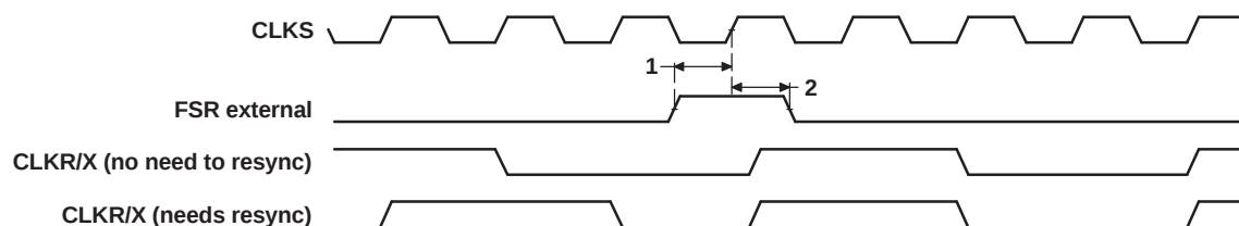
Figure 6-26. FSR Timing When GSYNC = 1
