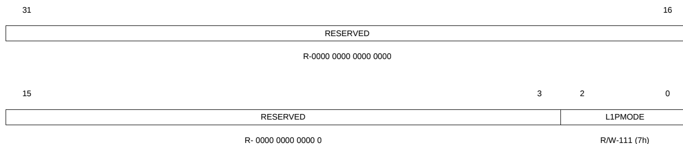
Figure 2-2. L1PCFG Register
