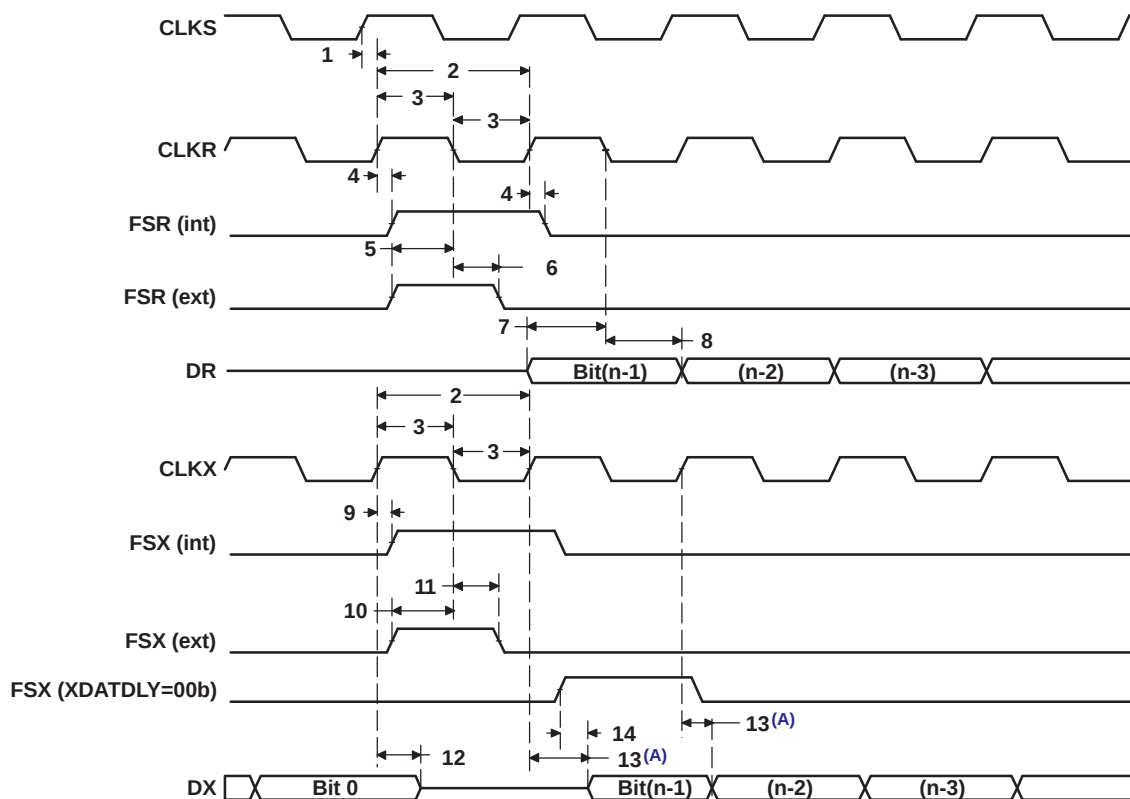
Figure 5-51. McBSP Timing
