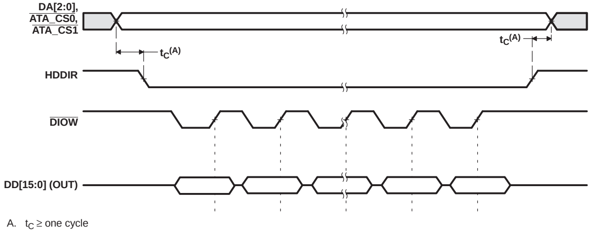
Figure 7-78. ATA HDDIR PIO Postwrite Start Timing
