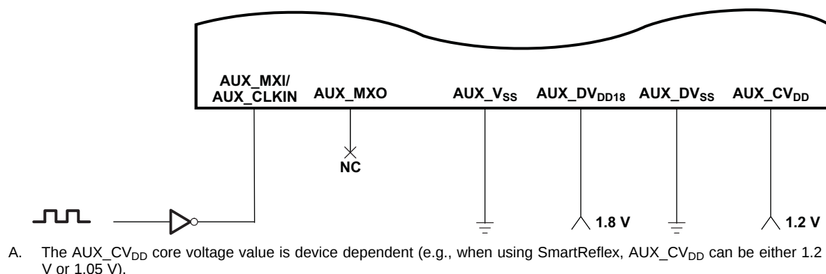
Figure 7-11. 1.8-V LVC MOS-Compatible Clock Input (A)
