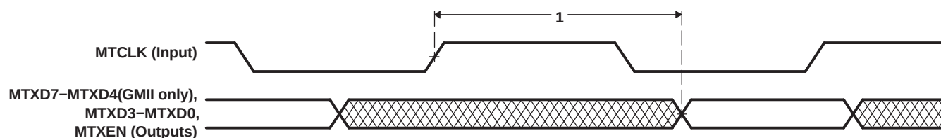
Figure 7-55. EMAC Transmit Interface Timing [MI and GMII Operation]
