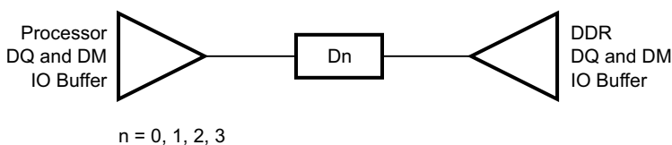
Figure 9-34. DQ/DM Topology
