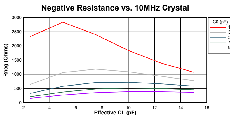
Figure 6-19. Negative Resistance Variation at 10 MHz
