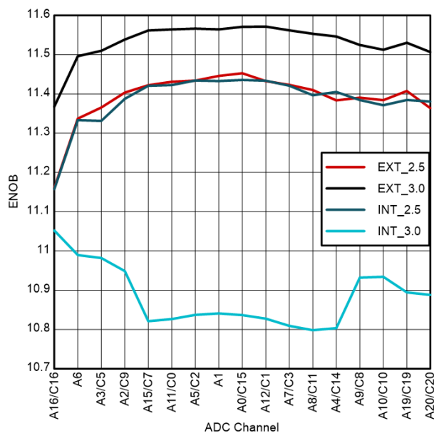
Figure 6-43. Per-Channel ENOB for 48-Pin RGZ VQFN
