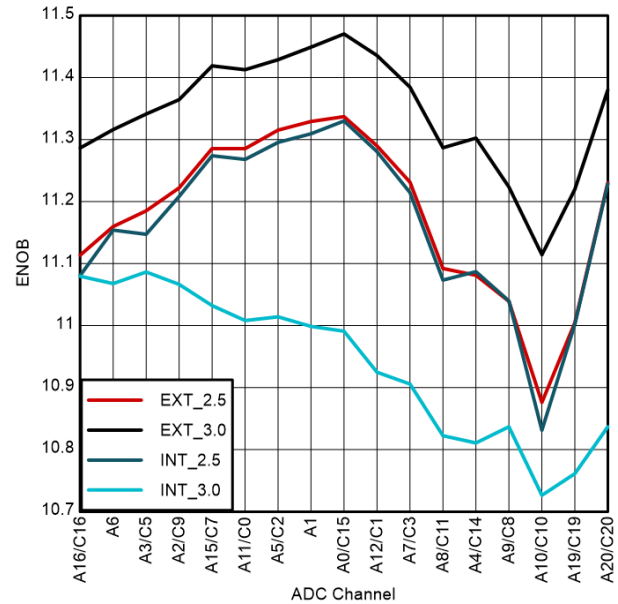
Figure 6-42. Per-Channel ENOB for 48-Pin PT LQFP
