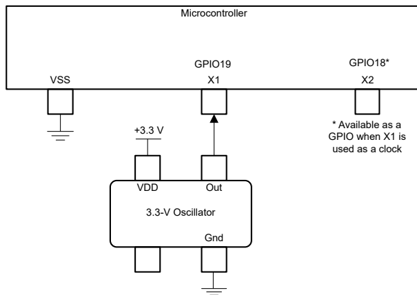
Figure 6-14. Single-ended 3.3-V External Clock
