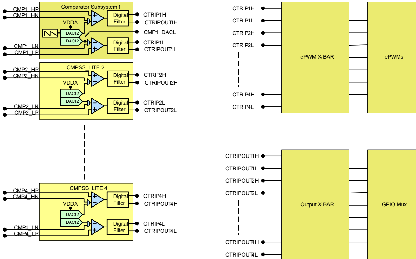
Figure 6-47. CMPSS Connectivity
