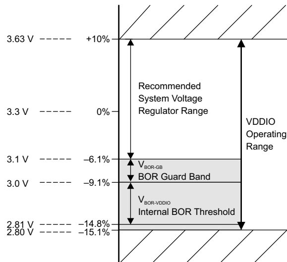
Figure 6-8. Supply Voltages
