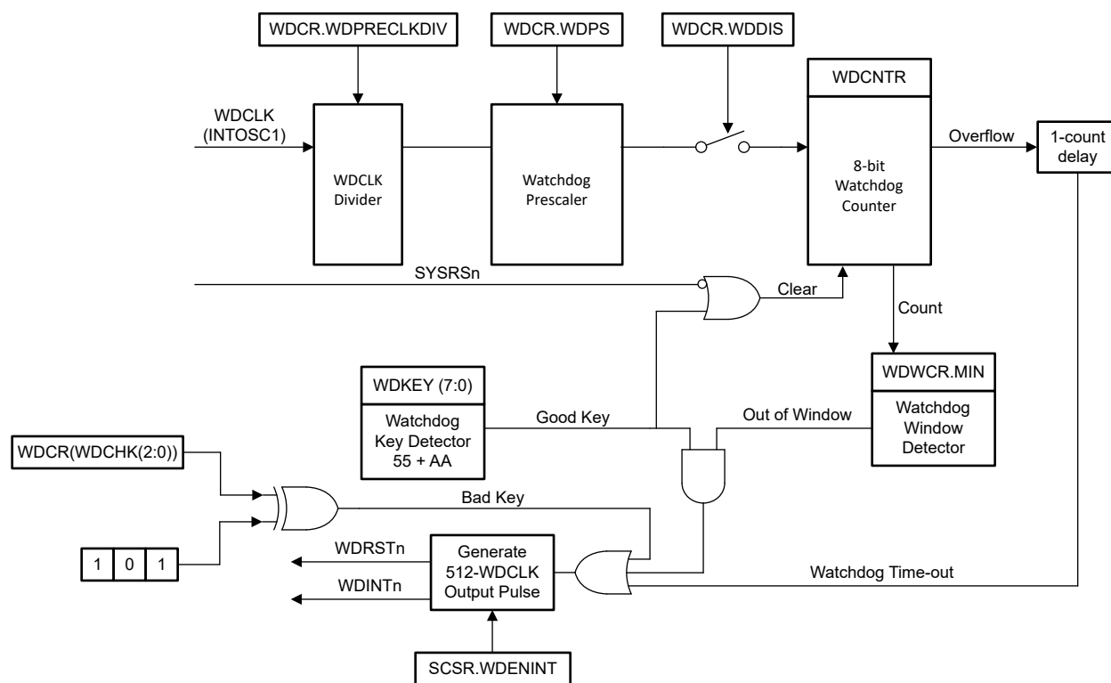
Figure 7-2. Windowed Watchdog
