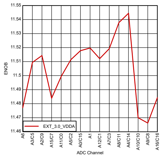
Figure 6-44. Per-Channel ENOB for 32-Pin RHB VQFN
