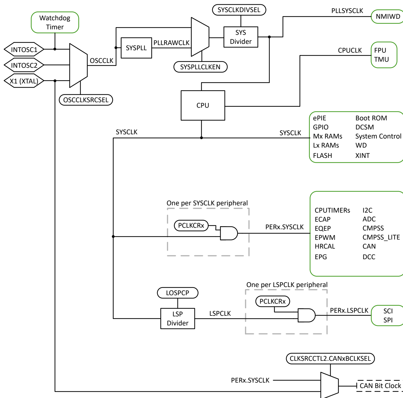
Figure 6-12. Clocking System
