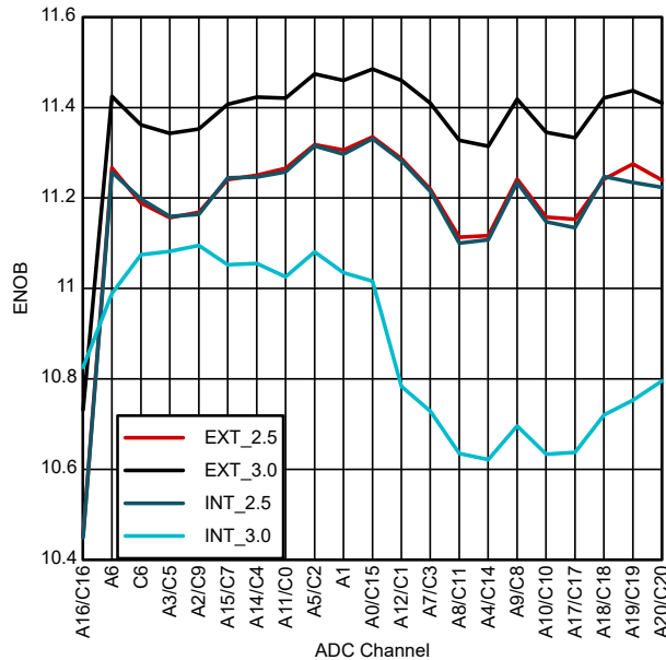
Figure 6-41. Per-Channel ENOB for 64-Pin PM LQFP
