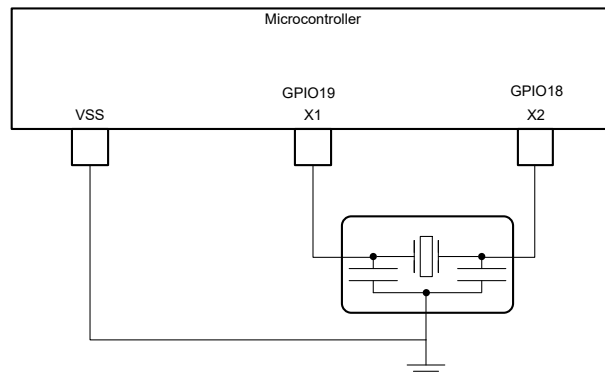
Figure 6-16. External Resonator
